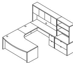
Right U w/Corner + Storage 108x102 KENTYP15R 70.1 cu.ft. - 797 lbs. Consists of: KEN-87R,65,93, 43,75,44,12,55
