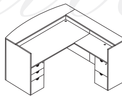
Reception Station 72x72x43H KENTYP19 37.2 cu.ft. - 472 lbs. Consists of: KEN-122,65, 125,75,124
